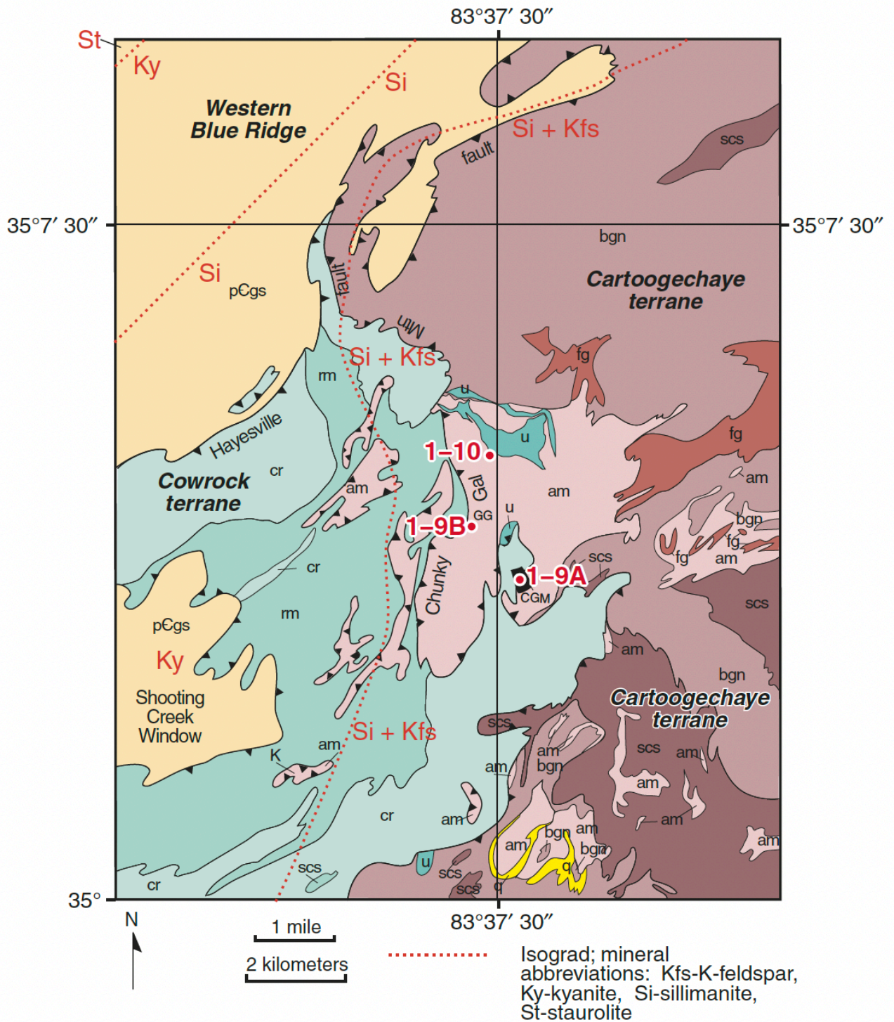
Figure 13. Detailed geologic map of the area near Chunky Gal Mountain (Stop 9A) and Glade Gap (Stop 9B), Shooting Creek and Rainbow Springs quadrangles. am—amphibolite; bgn—quartz-plagioclase-biotite gneiss; CGM—Chunky Gal Mountain; cr—Coleman River Formation, Coweeta Group; fg— felsic gneiss (possible 1.1 Ga basement gneiss); GG—Glade Gap; p Cgs—Great Smoky Group; q— Rainbow Springs quartzite; rm— Ridgepole Mountain Formation, Coweeta Group (mostly biotite and muscovite schist); scs—Shooting Creek schist; u—ultramafic rocks. Geology by RDH, assisted by Gregory Bryan, Stephen C. Godfrey, Louis L. Acker, and Brad Hubbard, 1977–1978.
