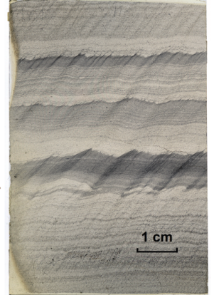
Wilhite Slate graded beds, US 64
