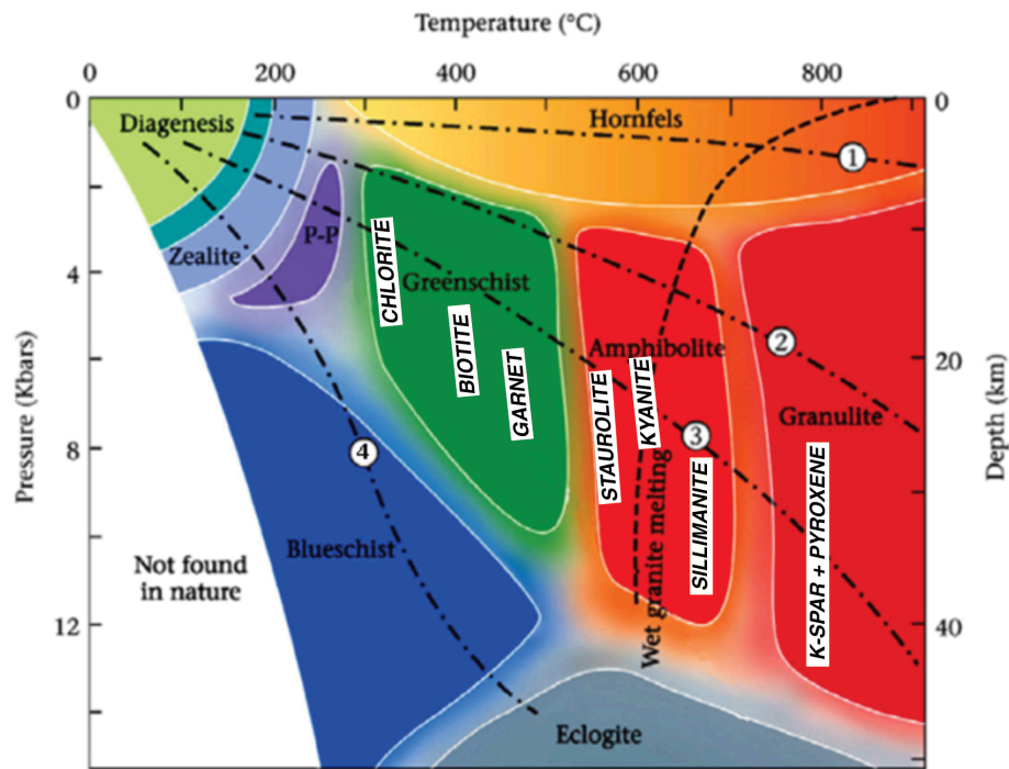
Figure 2. Correlation of T and P (depth) with the minerals we will see that tell us where we are in the crust on our traverse.
