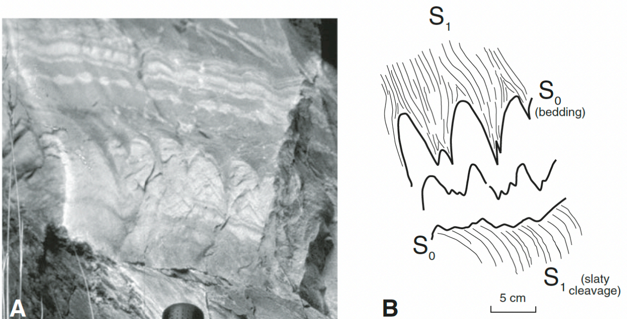
Figure 18. (A) Flattened ripples and refracting cleavage in Wilhite Formation slate (darker color) and interlayered silty carbonate (ankeritic dolomite) and fine-grained sandstone (light colored). (B) Relationships between flattened ripple marks in bedding and slaty cleavage at Madden Branch.
